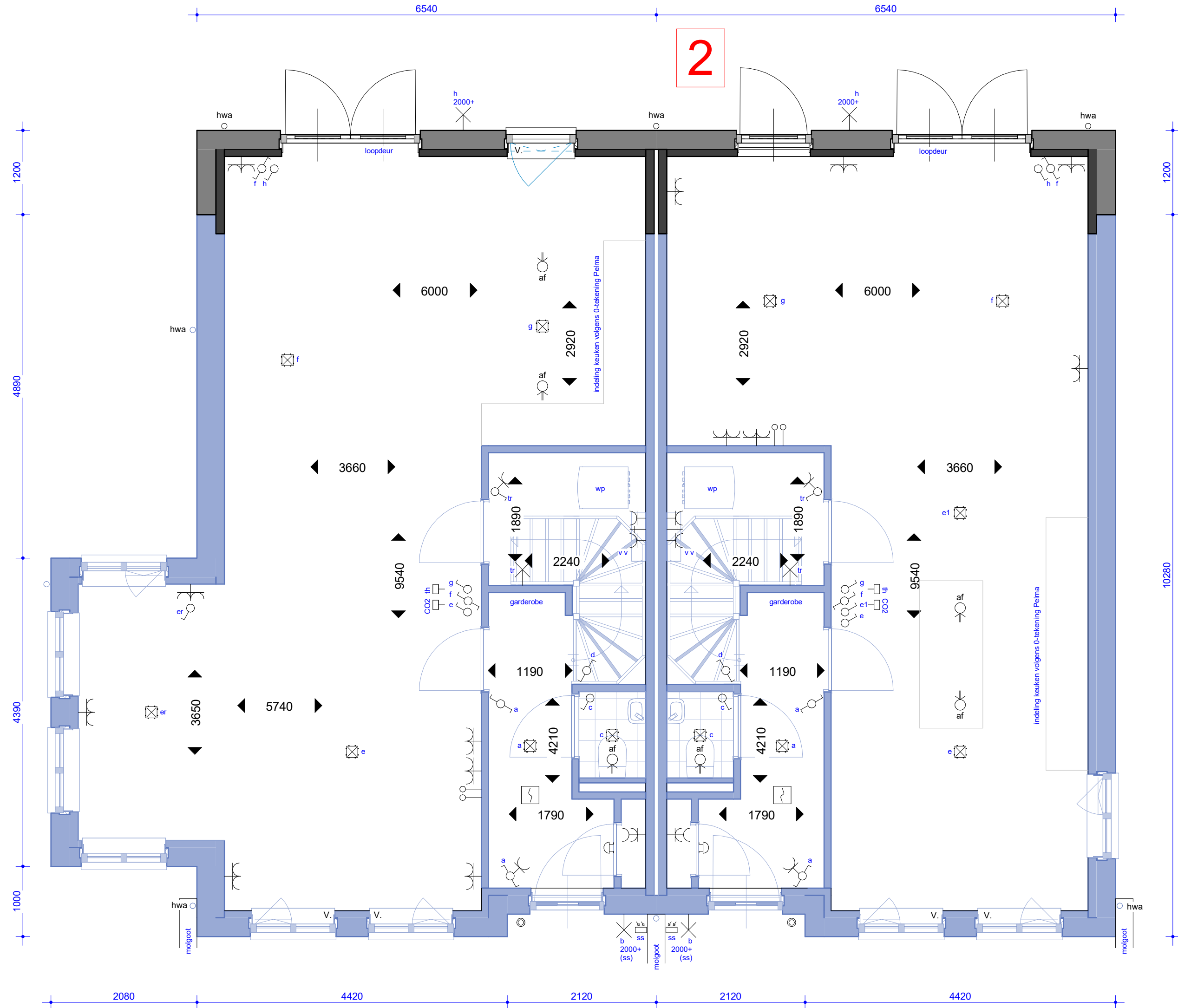
1 BEGANE GROND
