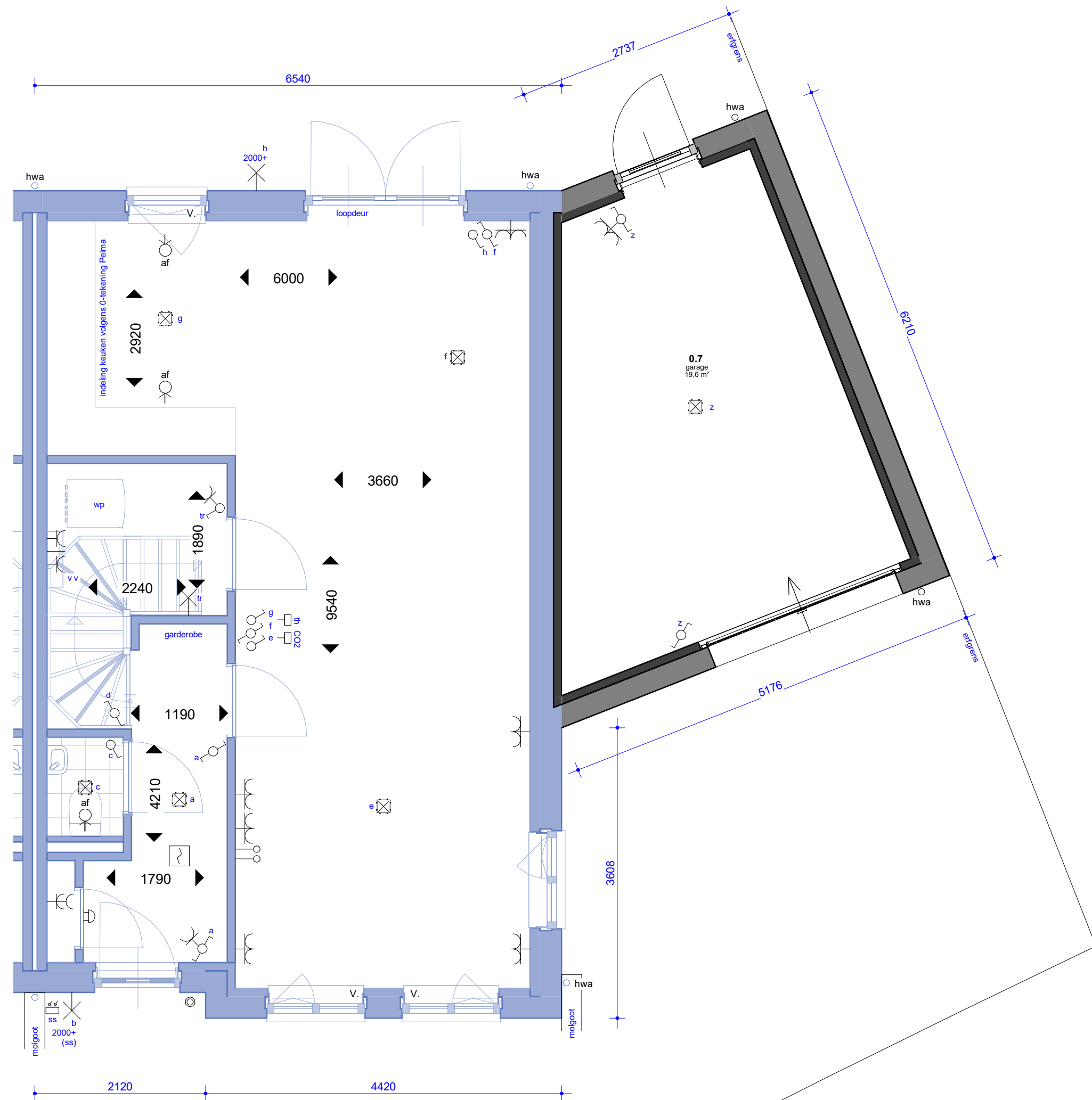
7 BEGANE GROND
